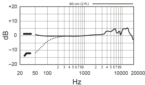
Frequency Response
